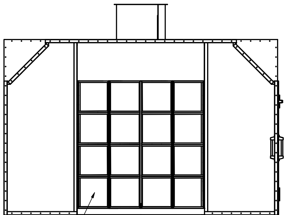
SECTION A-A SCALE 1 / 35
