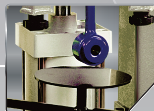
Lower Support Plate Holds strut when upper cap is unscrewed, prevents it from falling down. Allows for full use of both hands.
