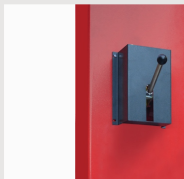
• Single point safety release makes it easier for operators to unlock both columns locks from one column.
