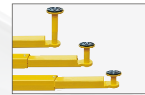
Standard drop-in adaptors 1.5", 2.5" & 5" extension high adaptors to fit different trucks and lifting height.
