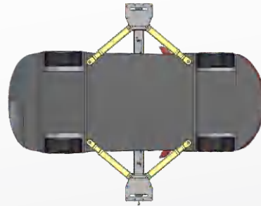
LOAD IN SYMMETRIC CONFIGURATION
