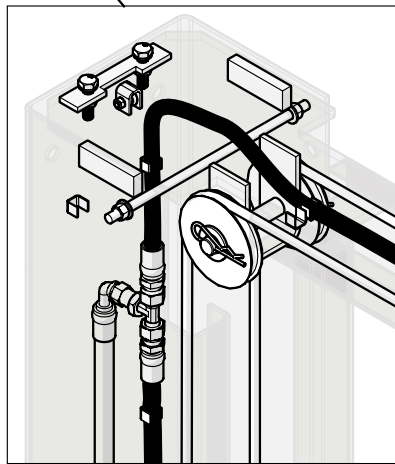
Power Side Post Bulkhead Tee Connections
